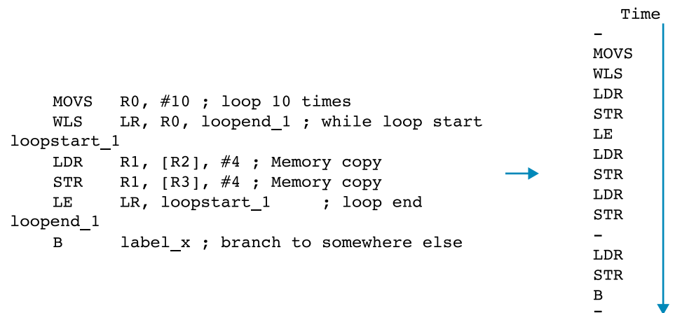
Fig. 8. Simple example of LOB instruction usage – memory copy
