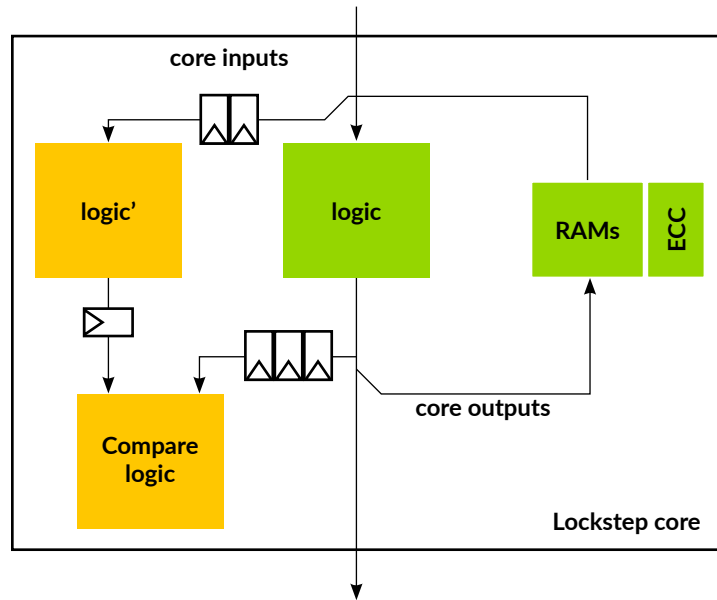
Figure 4: Dual Core LockStep processor with shared memories
