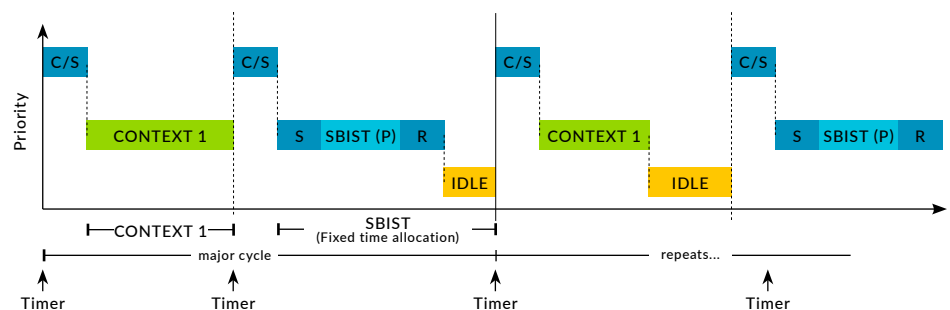
Figure 2: Use of a Software Test Library in a time triggered system
