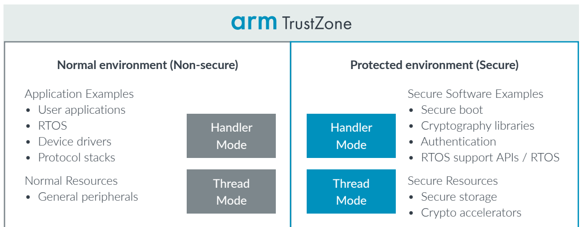
Figure 5 – Application components now need to be examined to determine if they are assets that need to be protected or are used to protect an asset. If they are, those components belong in the Secure execution environment. The remaining components can belong to the Non-secure application.
