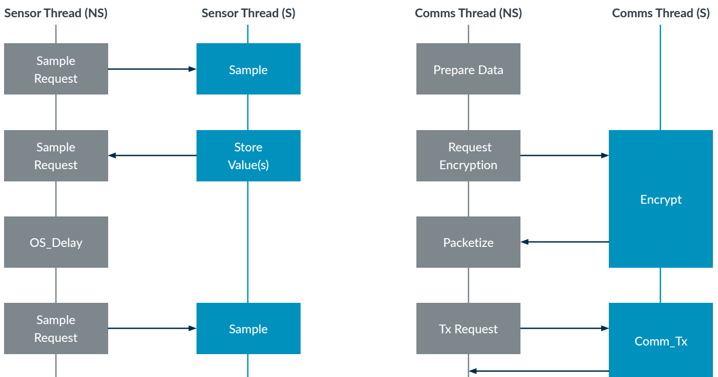
Figure 6 – Example sequence diagram for two application threads that have Secure and Non-secure function calls.
