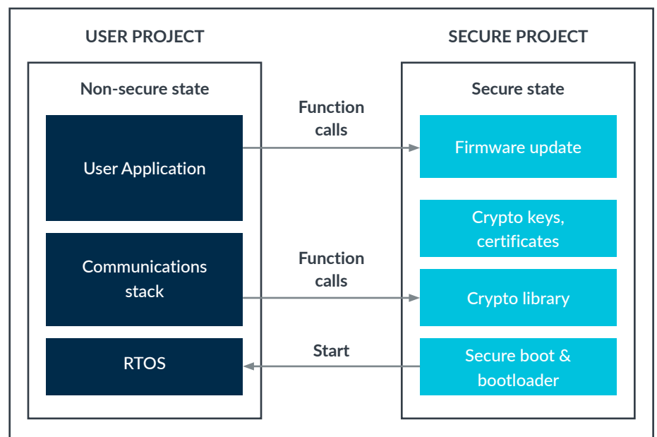
Figure 4 – A TrustZone application example
