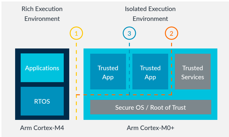
Figure 3 – An example implementation of security through isolation leveraging multiple processors on the same chip in the Cypress PSoC 64 Secure Microcontroller. (Source: Cypress)
