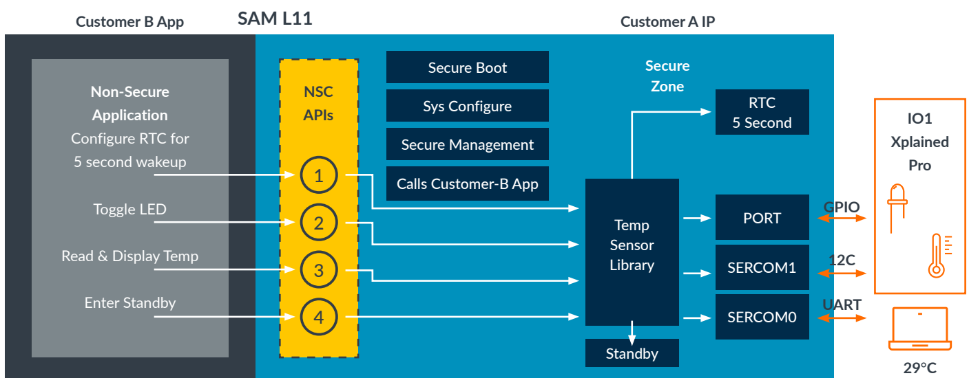
Figure 7 – An example application from Microchip using the TrustZone enabled SAM L11 demonstrates how you can partition the application for Secure and Non-secure run-time environments.
